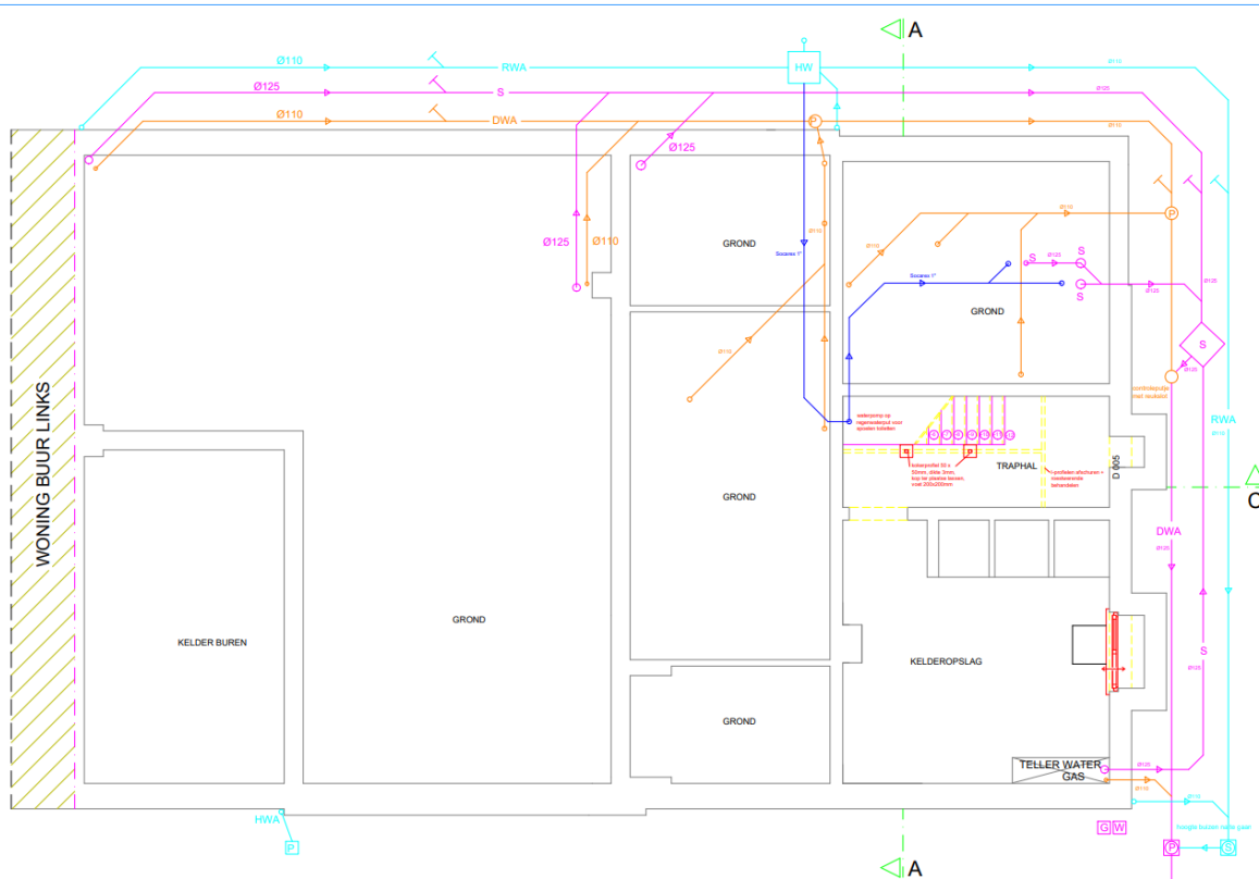
Plan kelder
